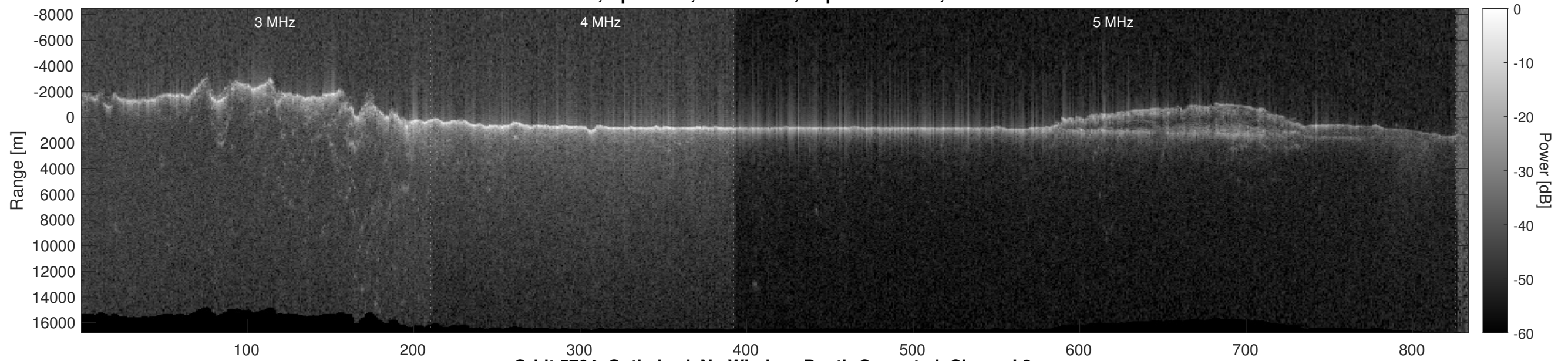
Orbit 5704, Optimized, No Window, Depth-Corrected, Channel 2
