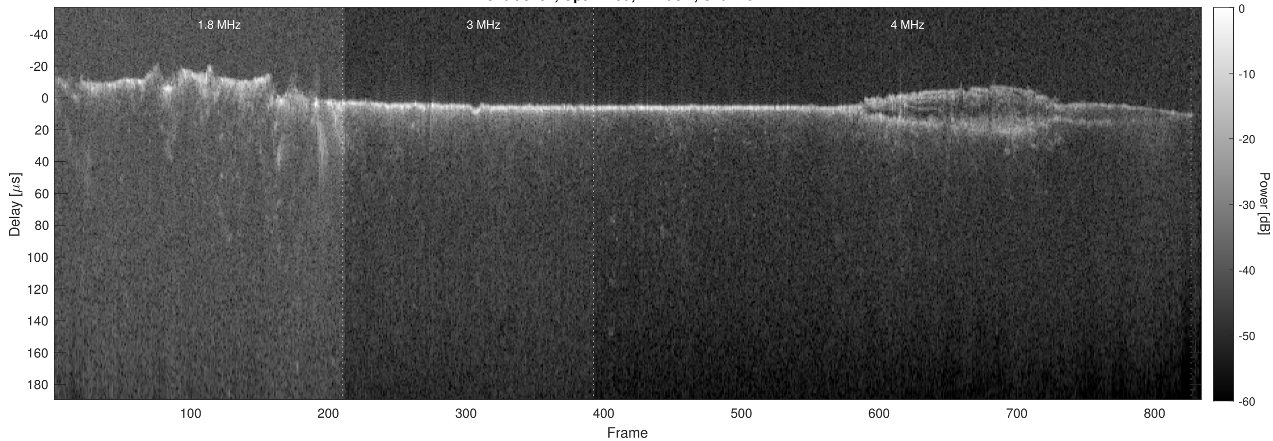
Orbit 5704, Optimized, Window, Channel 2
