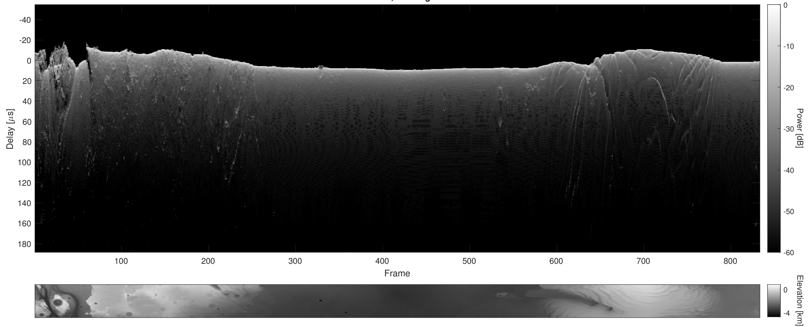
Orbit 5705, Cluttergram
