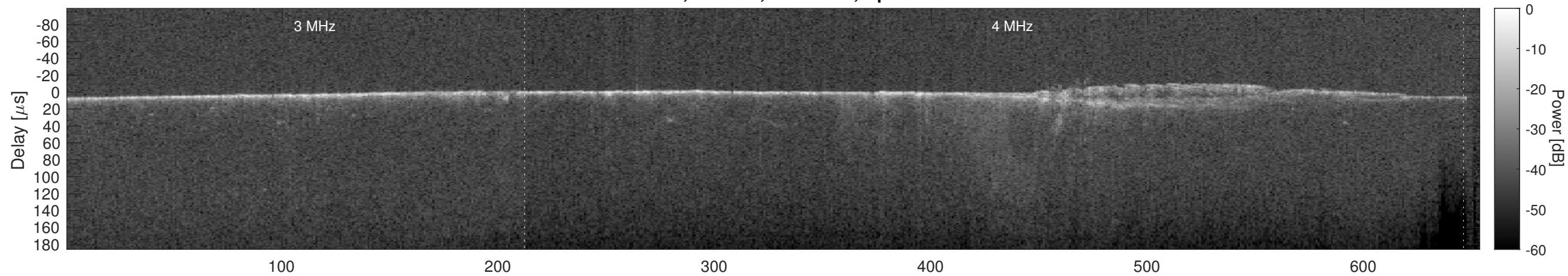
Orbit 5707, Cluttergram
