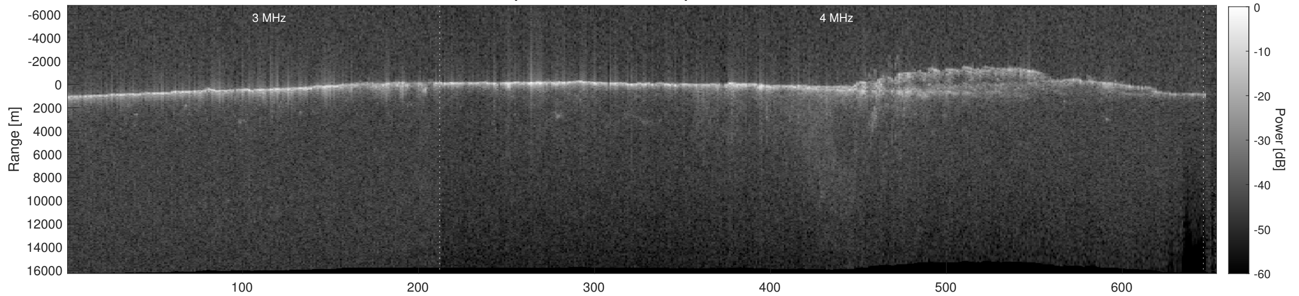
Orbit 5707, Depth-Corrected Cluttergram
