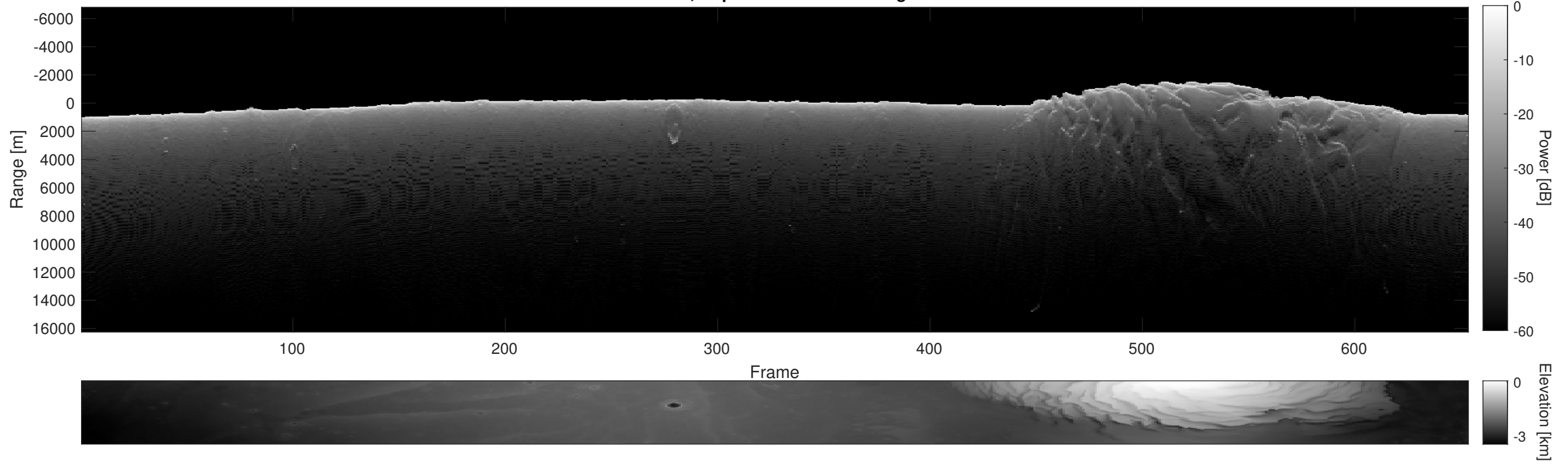
Orbit 5707, Depth-Corrected Cluttergram
