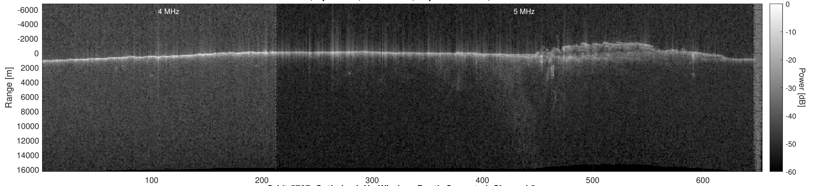
Orbit 5707, Optimized, No Window, Depth-Corrected, Channel 2
