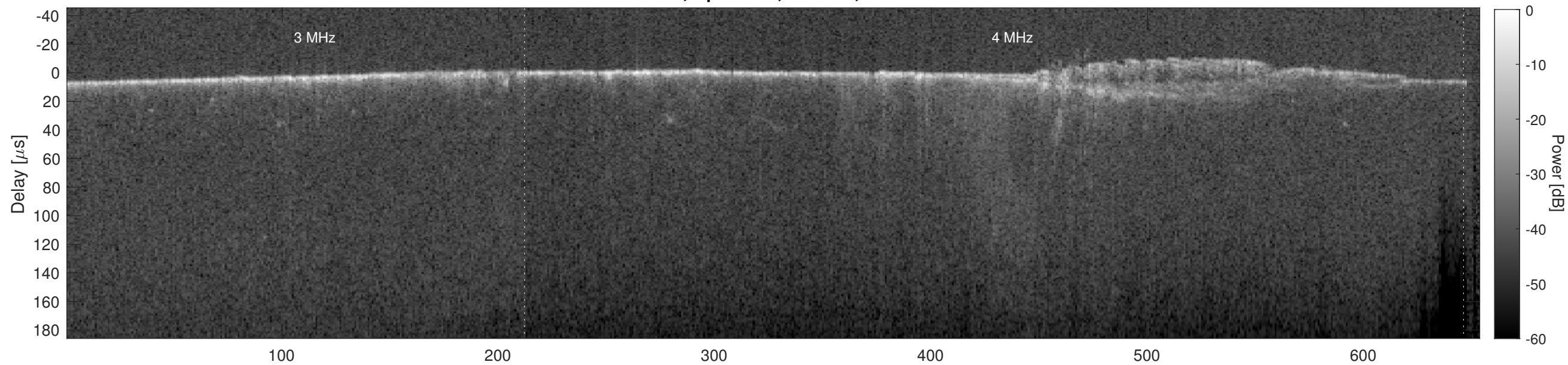
Orbit 5707, Cluttergram
