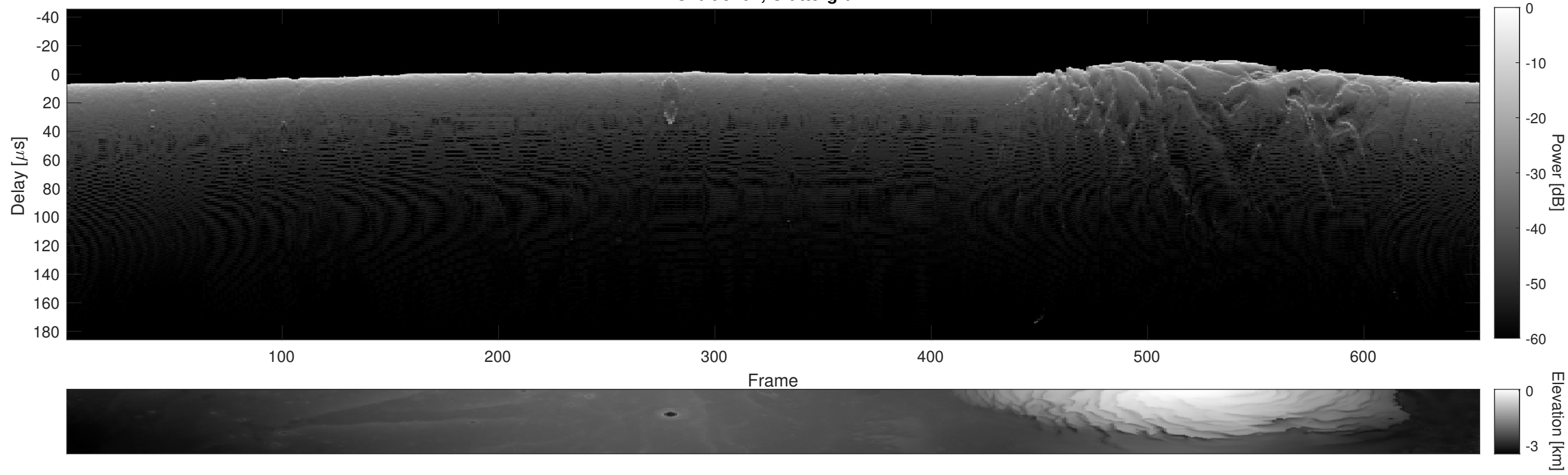
Orbit 5707, Cluttergram
