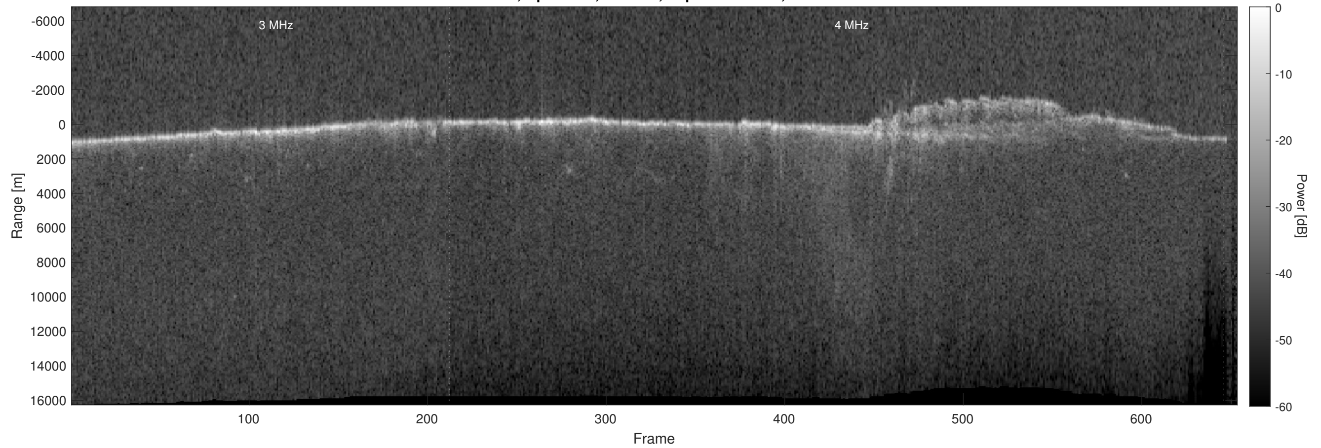
Orbit 5707, Optimized, Window, Depth-Corrected, Channel 2
