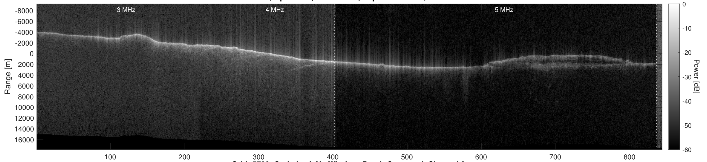
Orbit 5709, Optimized, No Window, Depth-Corrected, Channel 2
