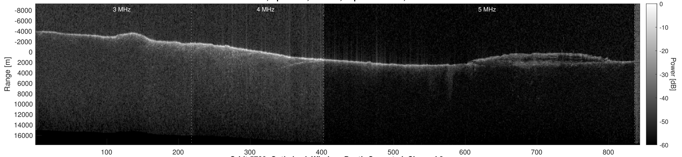
Orbit 5709, Optimized, Window, Depth-Corrected, Channel 2
