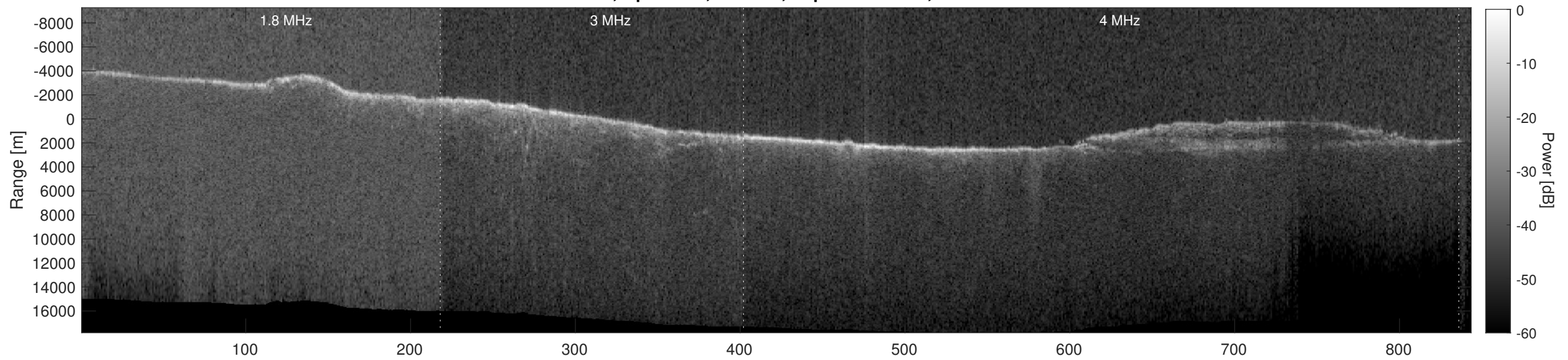
Orbit 5709, Depth-Corrected Cluttergram
