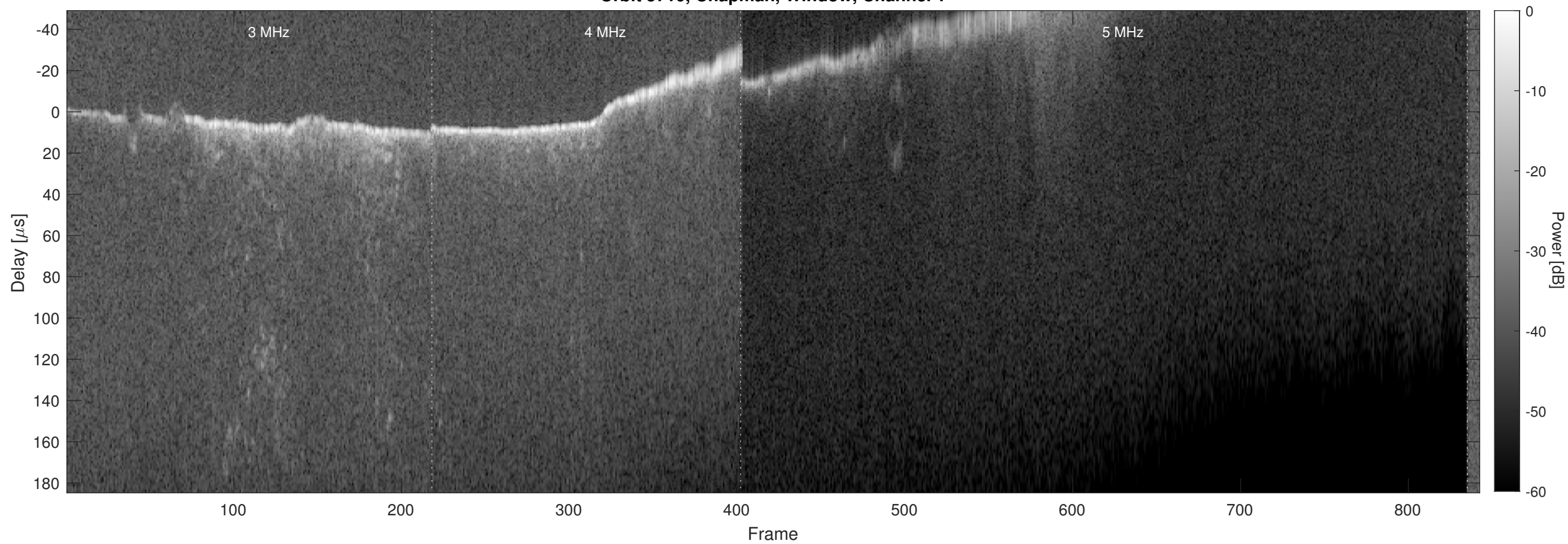
Orbit 5710, Chapman, Window, Channel 2
