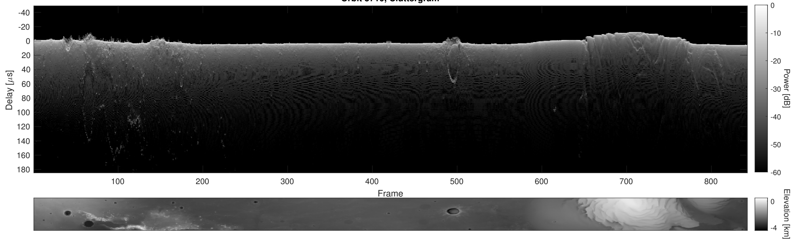
Orbit 5710, Cluttergram
