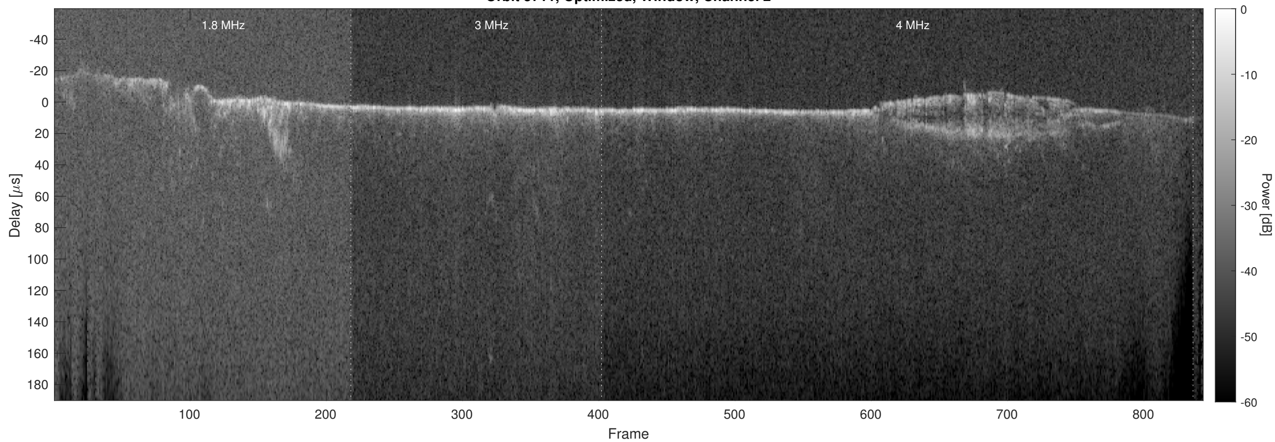
Orbit 5711, Optimized, Window, Channel 2
