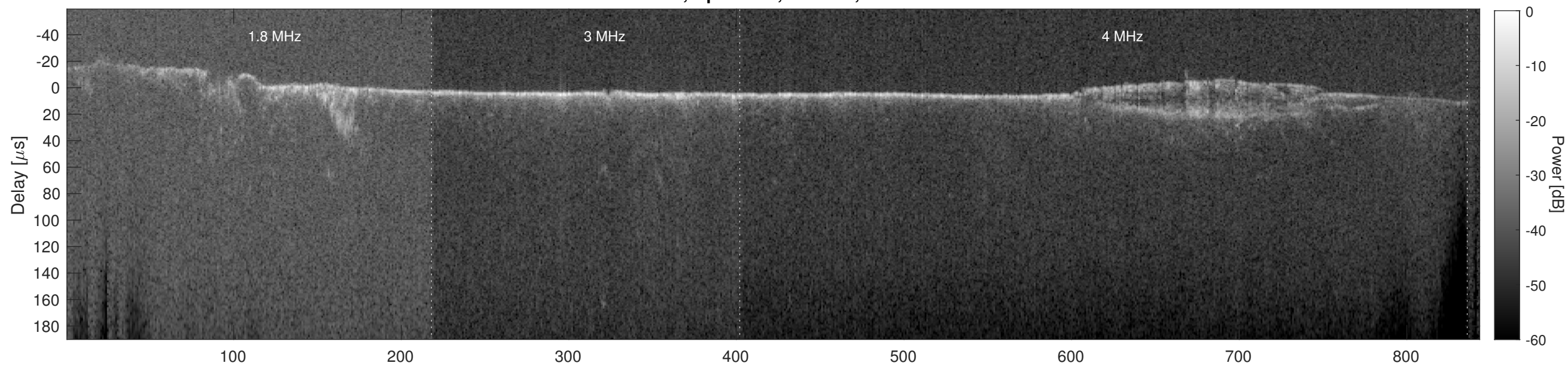
Orbit 5711, Cluttergram
