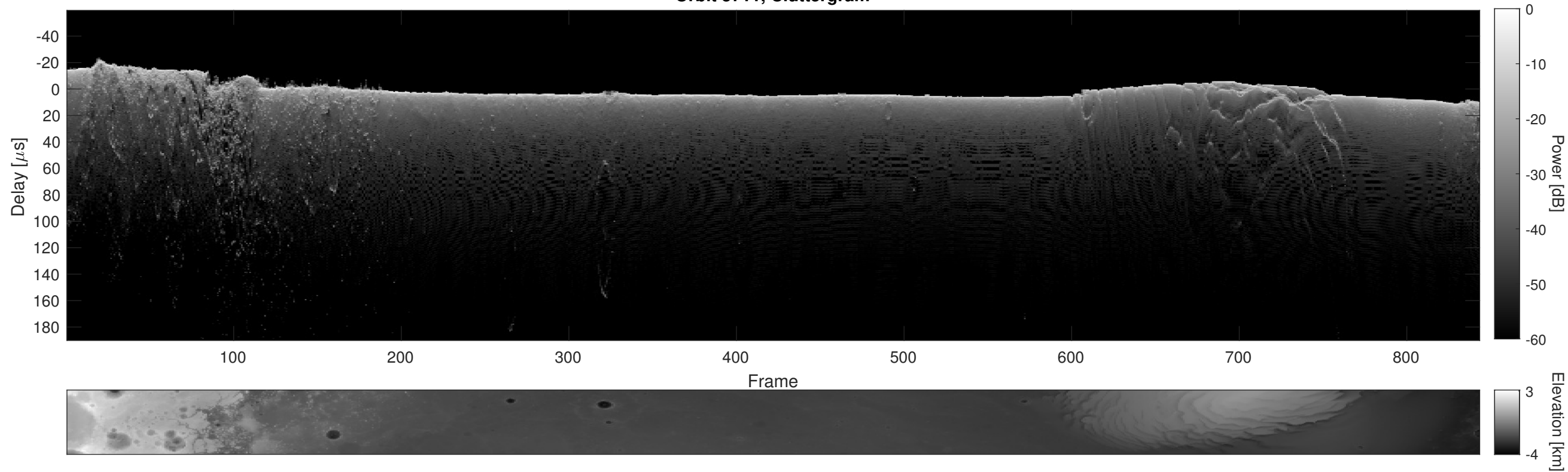
Orbit 5711, Cluttergram
