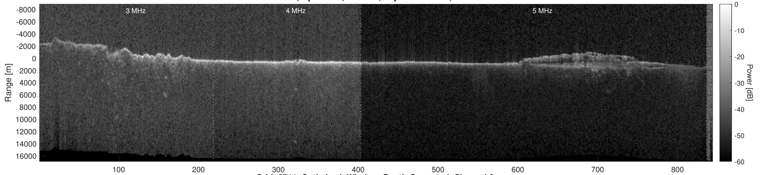
Orbit 5711, Optimized, Window, Depth-Corrected, Channel 2
