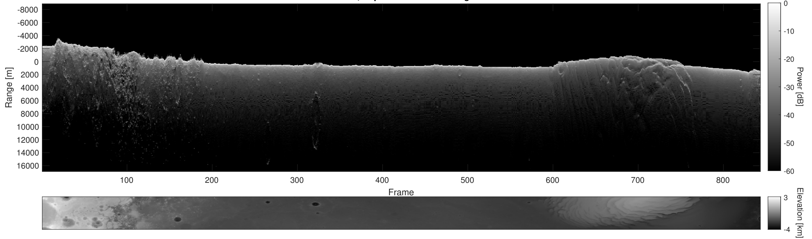
Orbit 5711, Depth-Corrected Cluttergram
