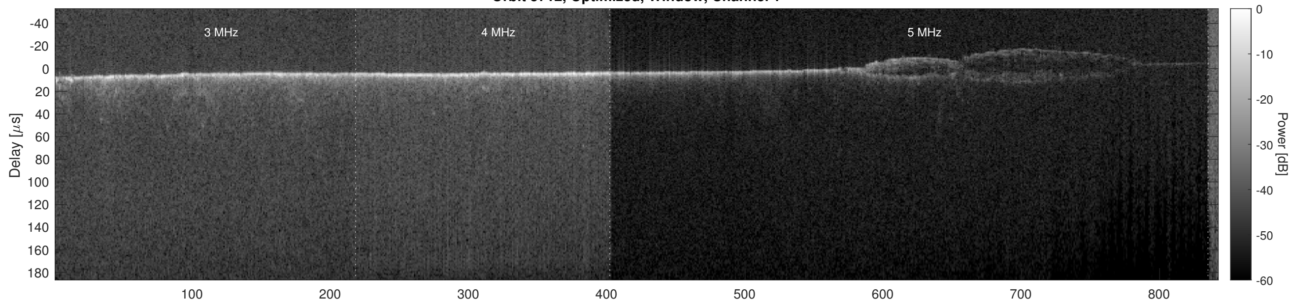
Orbit 5712, Optimized, Window, Channel 2
