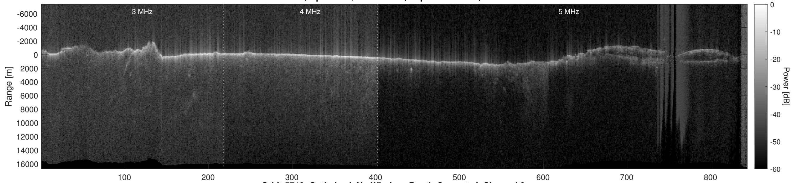
Orbit 5713, Optimized, No Window, Depth-Corrected, Channel 2
