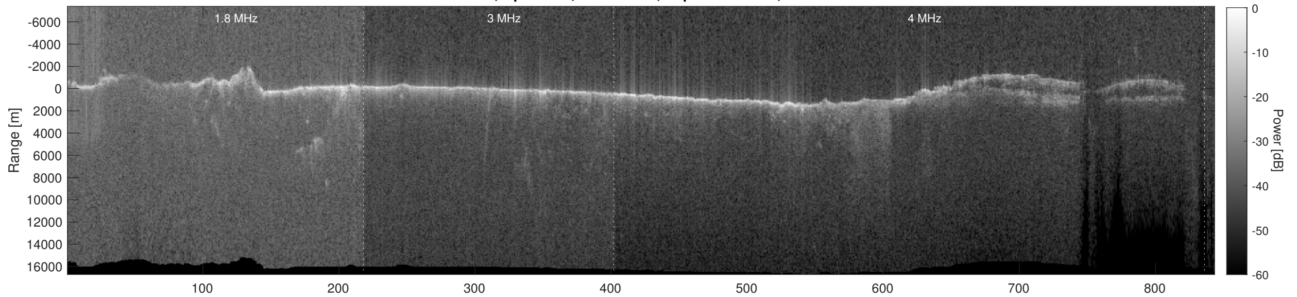
Orbit 5713, Depth-Corrected Cluttergram
