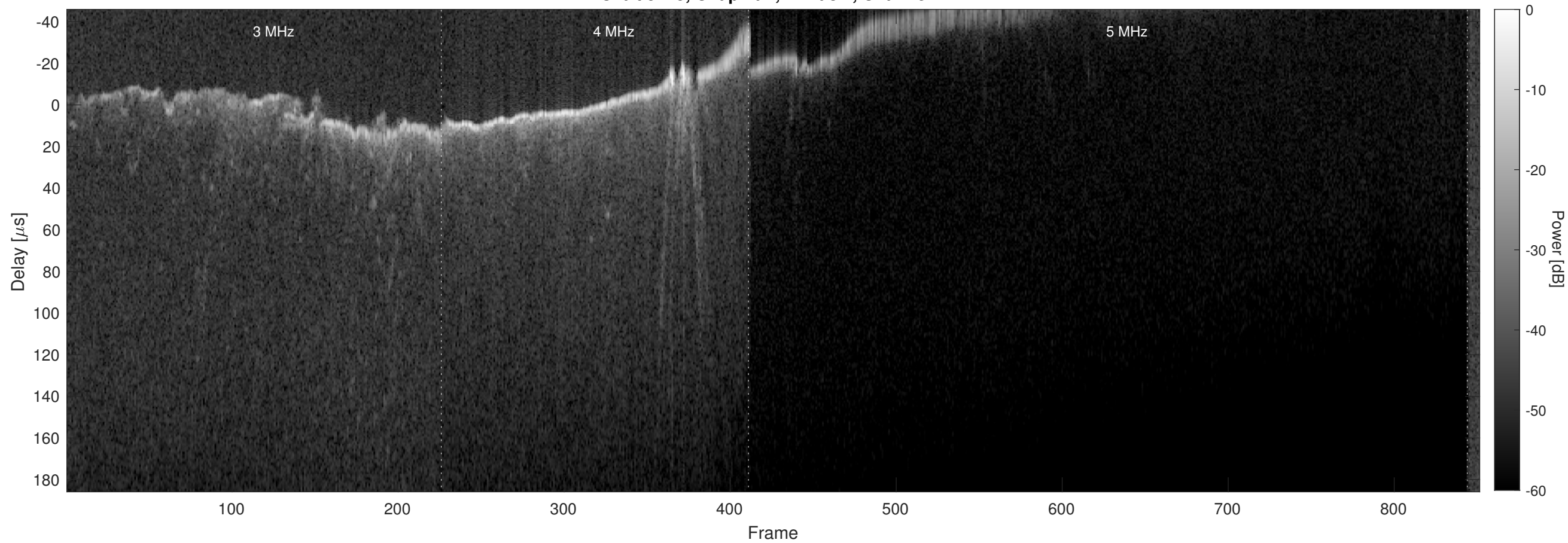
Orbit 5715, Chapman, Window, Channel 2
