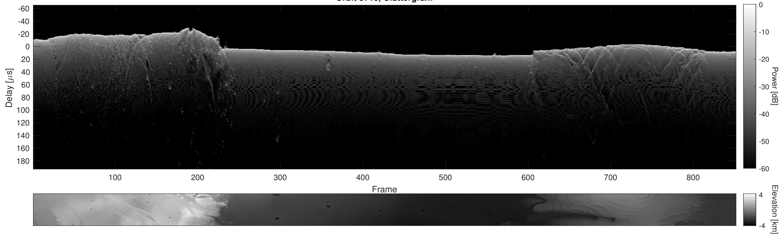
Orbit 5716, Cluttergram
