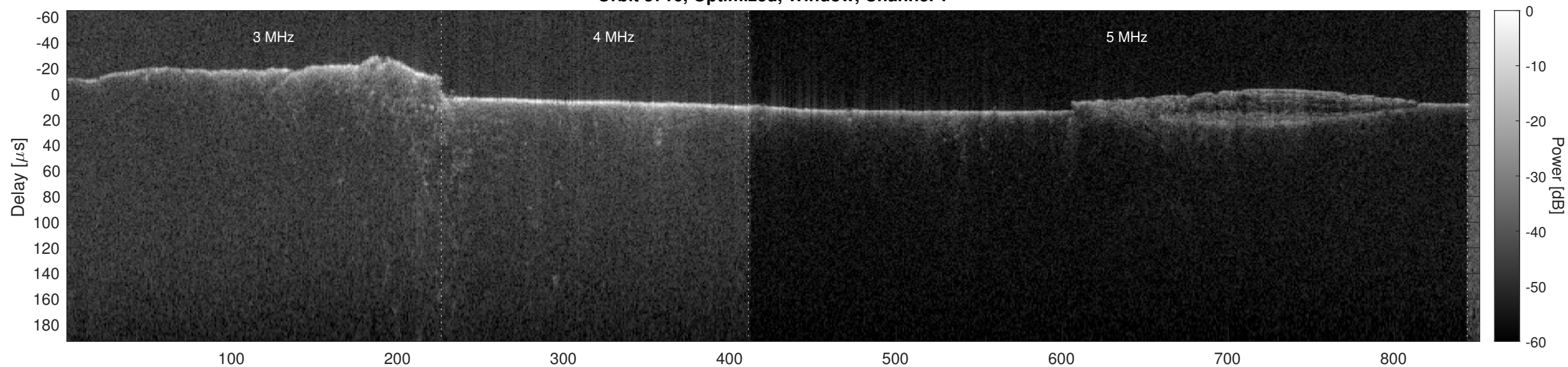
Orbit 5716, Optimized, Window, Channel 2
