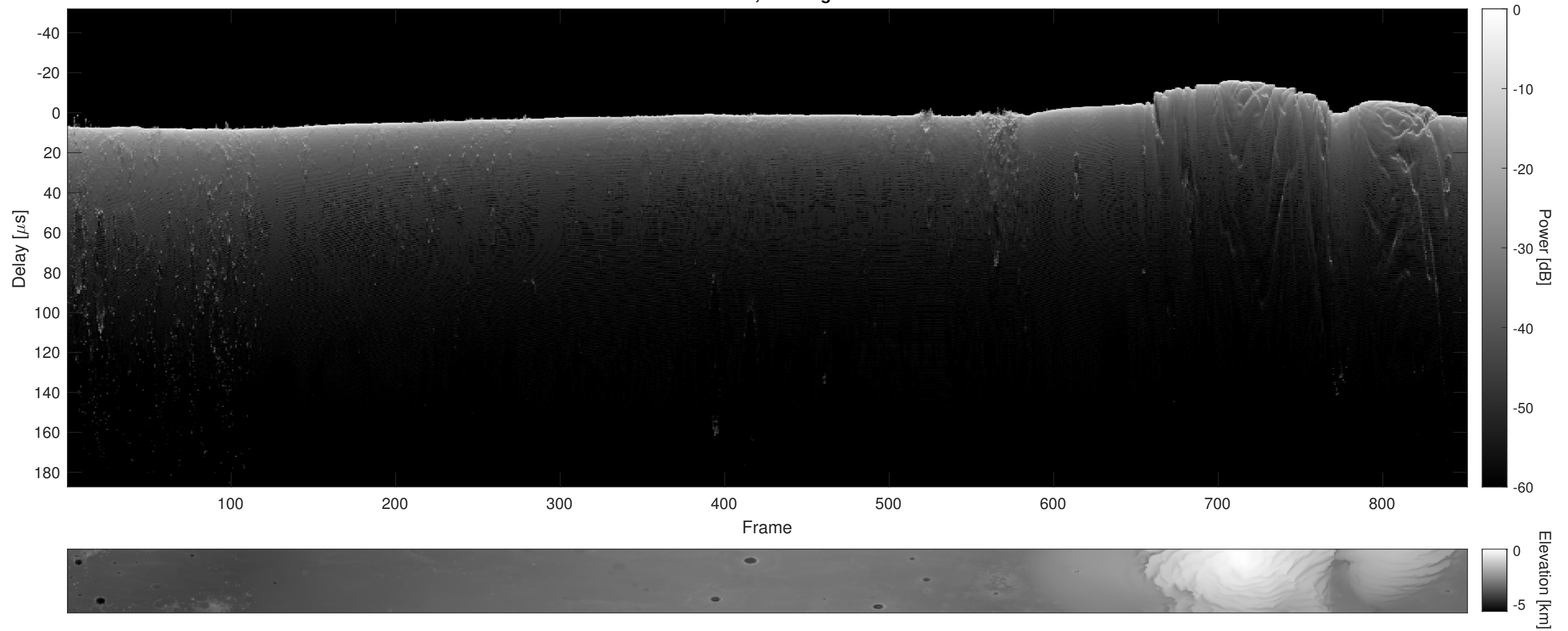
Orbit 5717, Cluttergram
