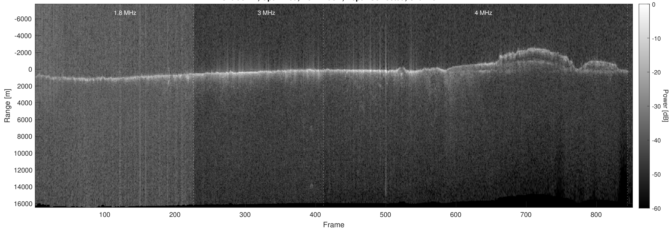
Orbit 5717, Optimized, No Window, Depth-Corrected, Channel 2
