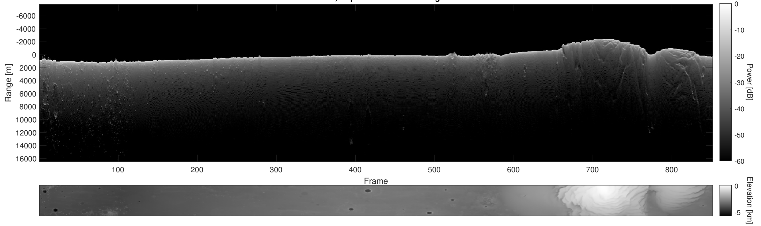
Orbit 5717, Depth-Corrected Cluttergram
