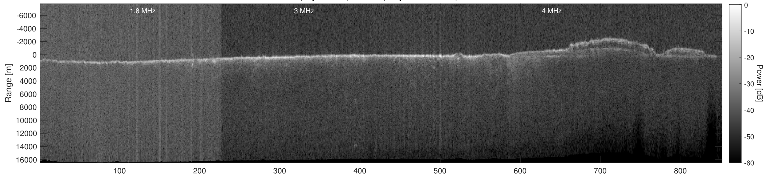
Orbit 5717, Depth-Corrected Cluttergram
