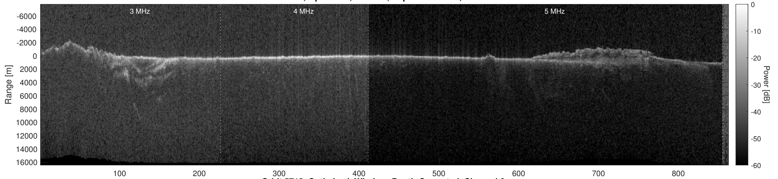
Orbit 5718, Optimized, Window, Depth-Corrected, Channel 2
