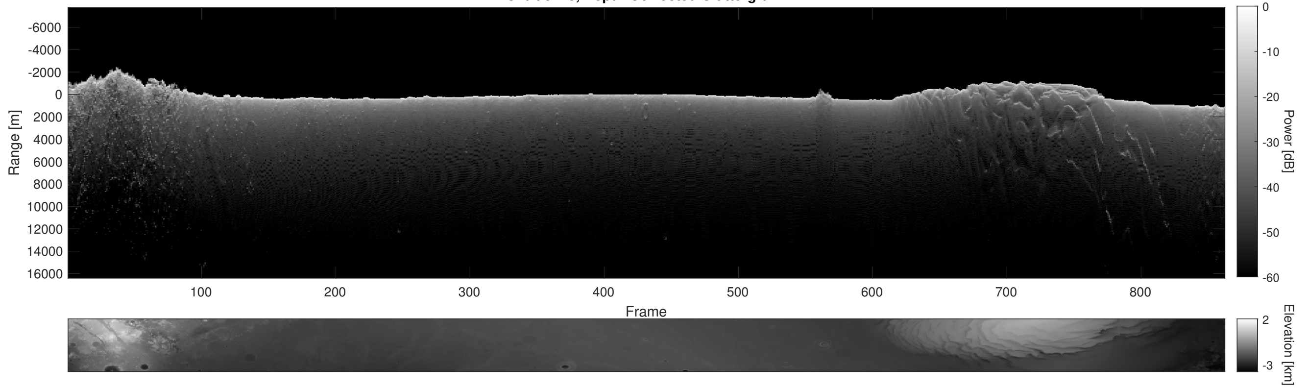
Orbit 5718, Depth-Corrected Cluttergram
