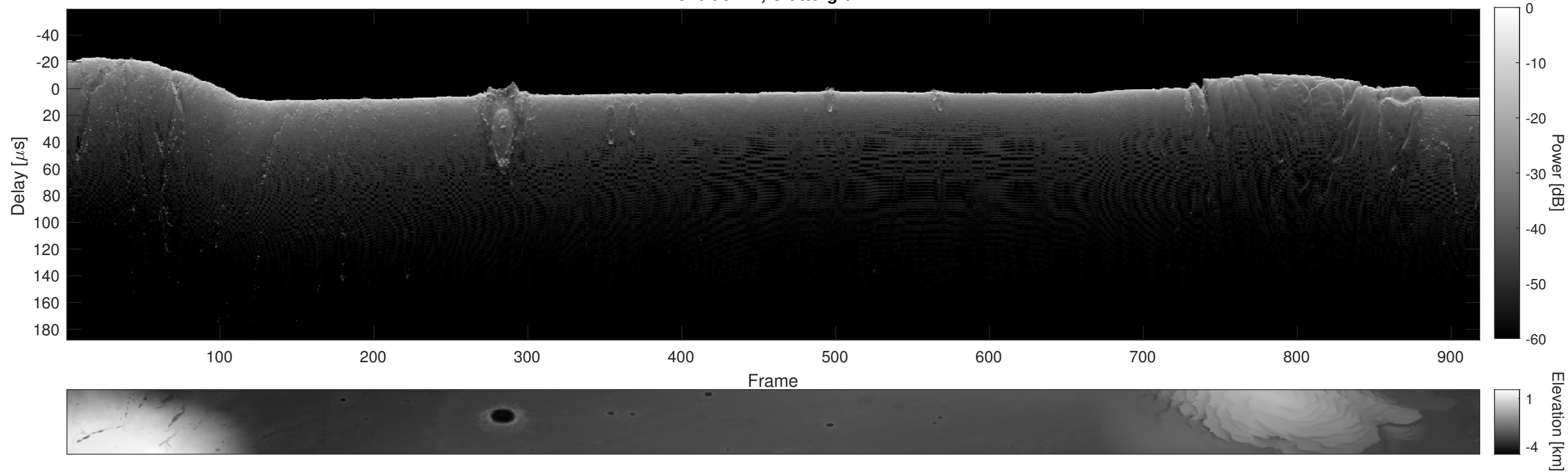
Orbit 5721, Cluttergram
