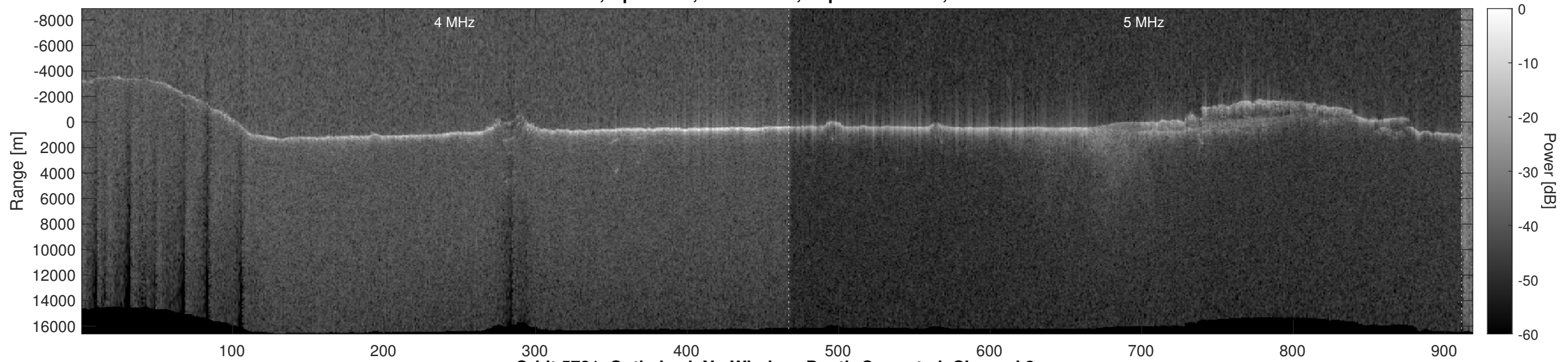
Orbit 5721, Optimized, No Window, Depth-Corrected, Channel 2
