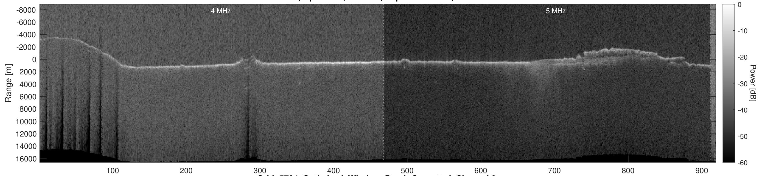
Orbit 5721, Optimized, Window, Depth-Corrected, Channel 2
