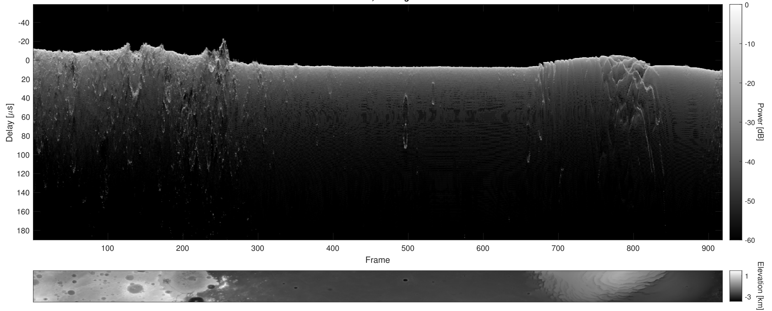
Orbit 5722, Cluttergram
