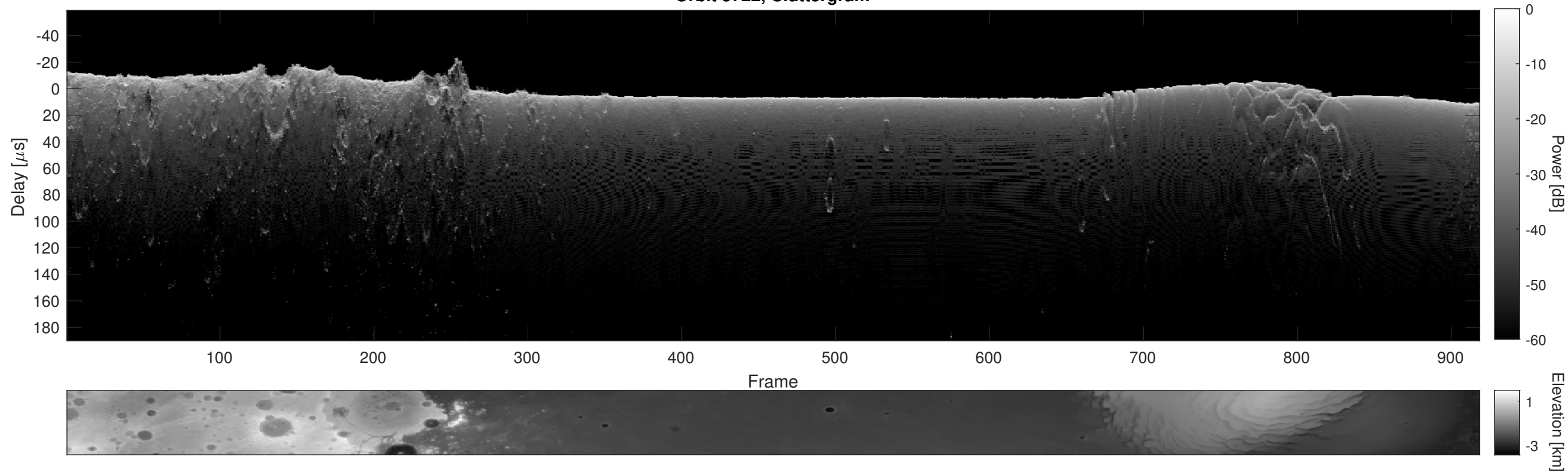
Orbit 5722, Cluttergram
