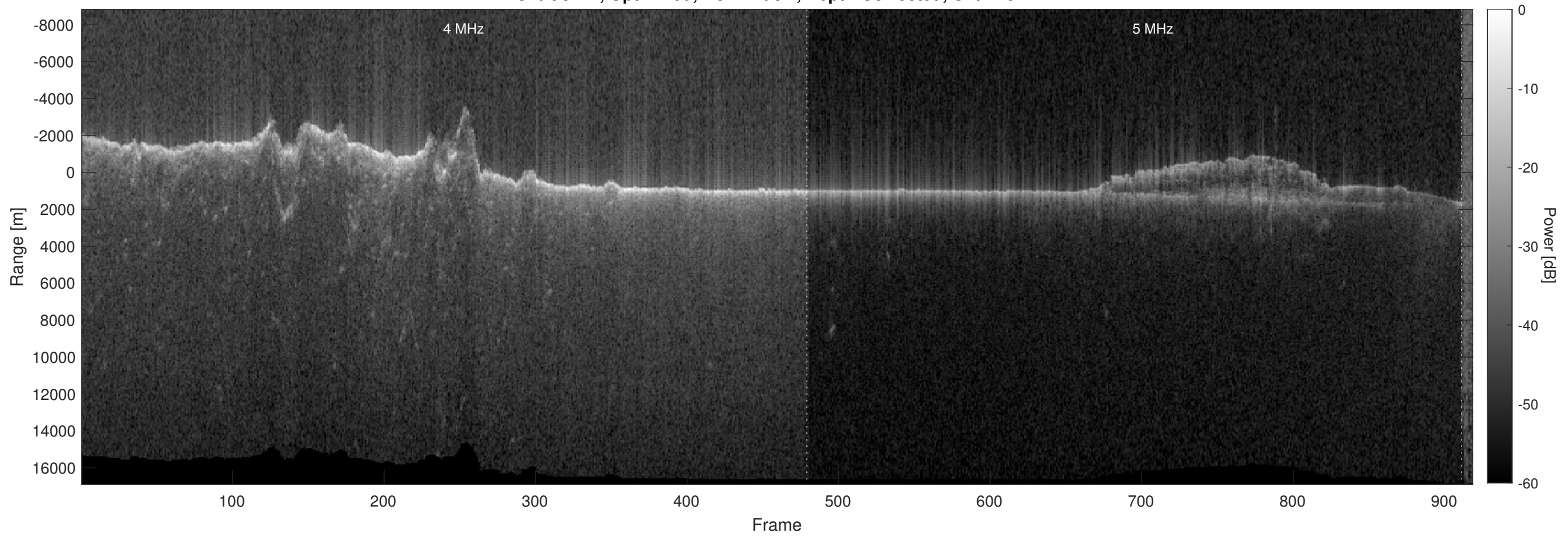
Orbit 5722, Optimized, No Window, Depth-Corrected, Channel 2
