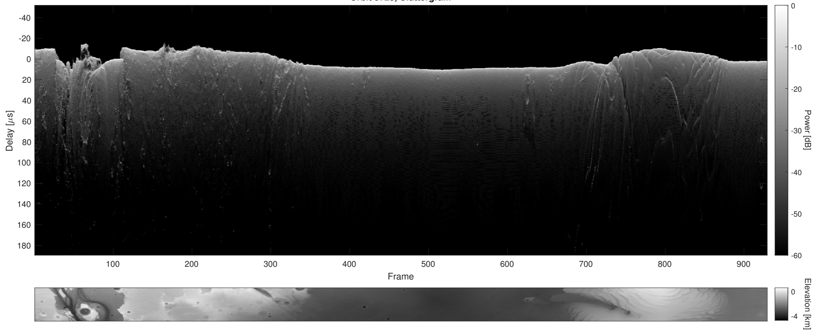
Orbit 5723, Cluttergram
