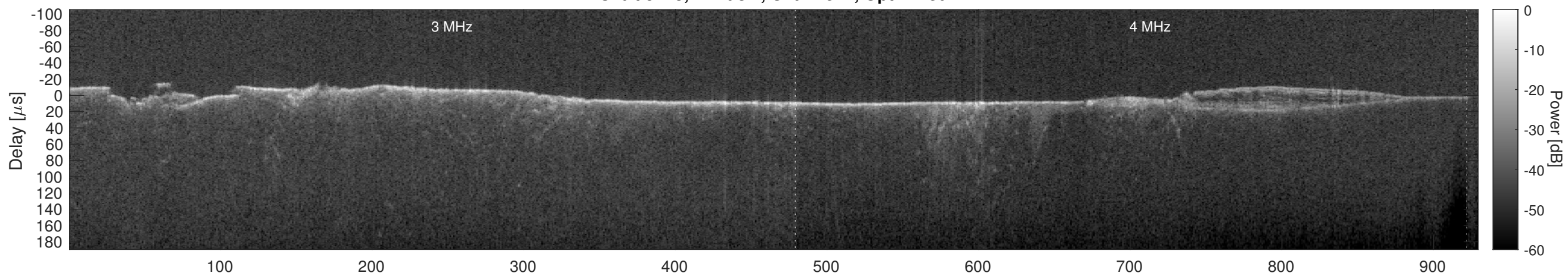
Orbit 5723, Cluttergram
