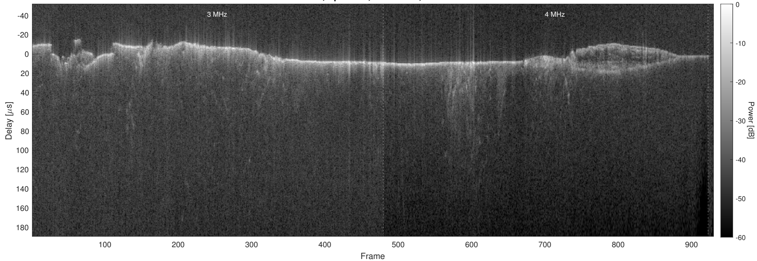
Orbit 5723, Optimized, No Window, Channel 2
