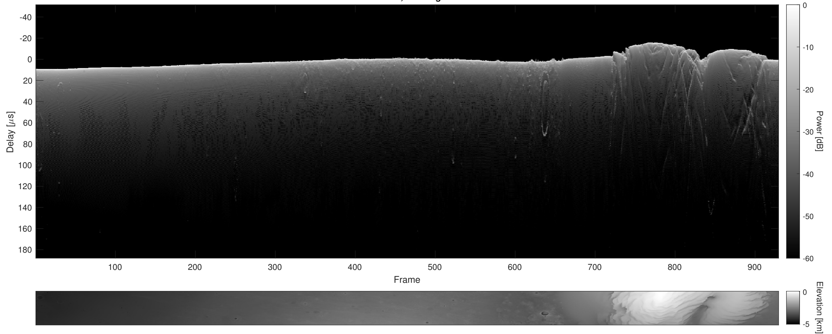
Orbit 5724, Cluttergram
