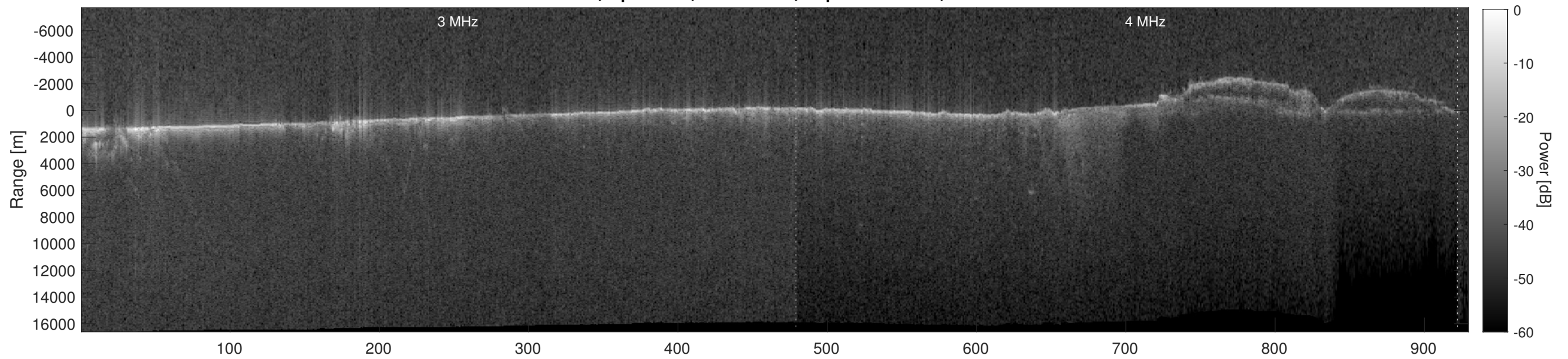
Orbit 5724, Depth-Corrected Cluttergram
