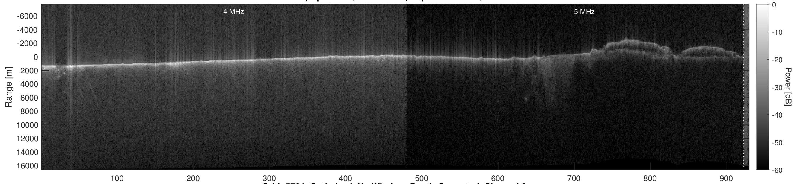
Orbit 5724, Optimized, No Window, Depth-Corrected, Channel 2
