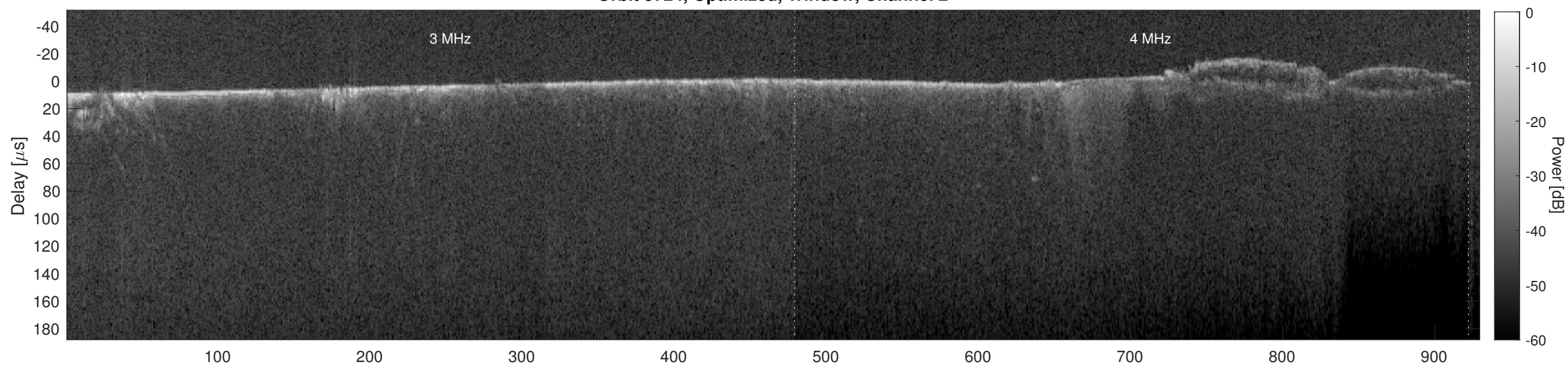
Orbit 5724, Cluttergram
