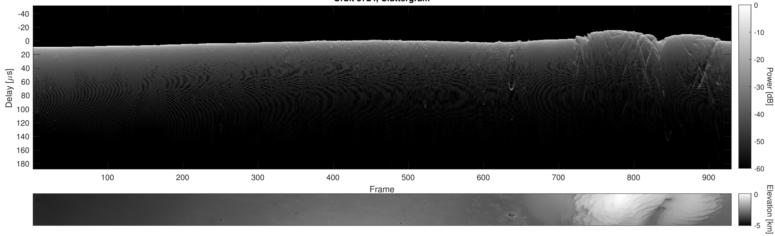
Orbit 5724, Cluttergram
