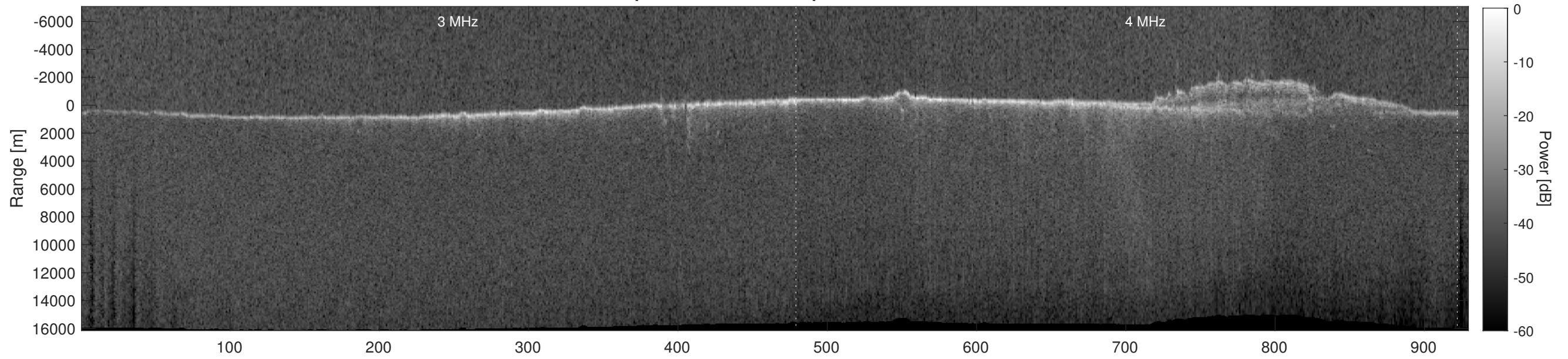
Orbit 5725, Depth-Corrected Cluttergram
