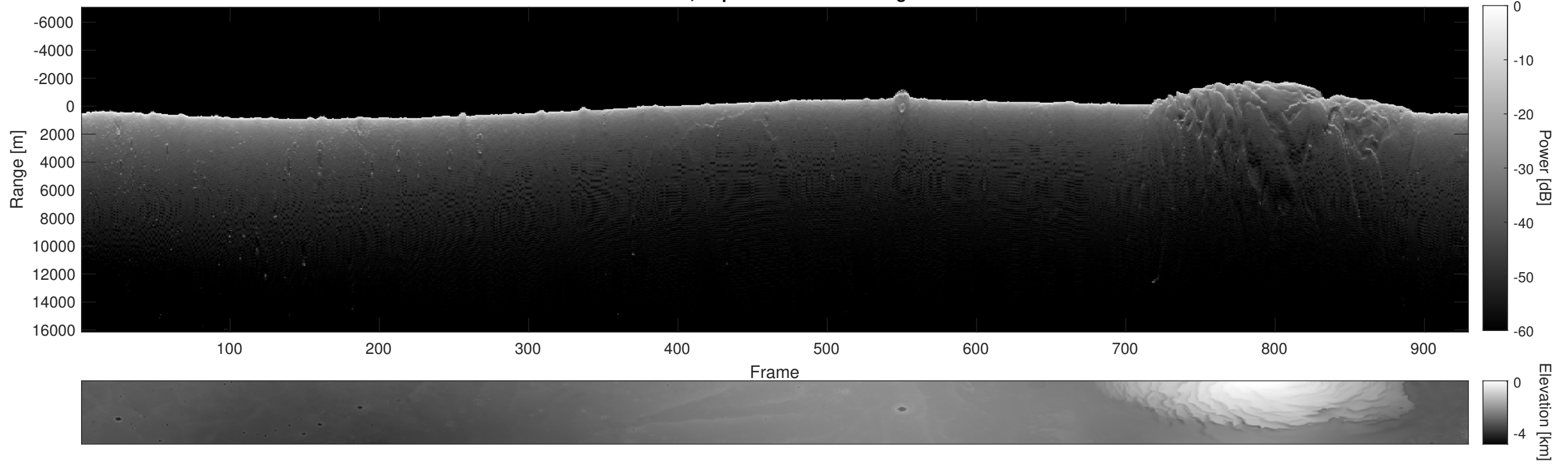
Orbit 5725, Depth-Corrected Cluttergram
