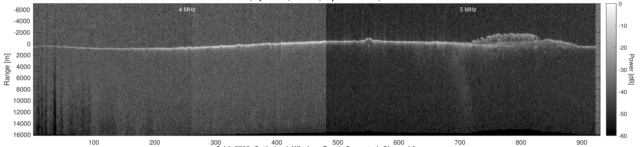
Orbit 5725, Optimized, Window, Depth-Corrected, Channel 2
