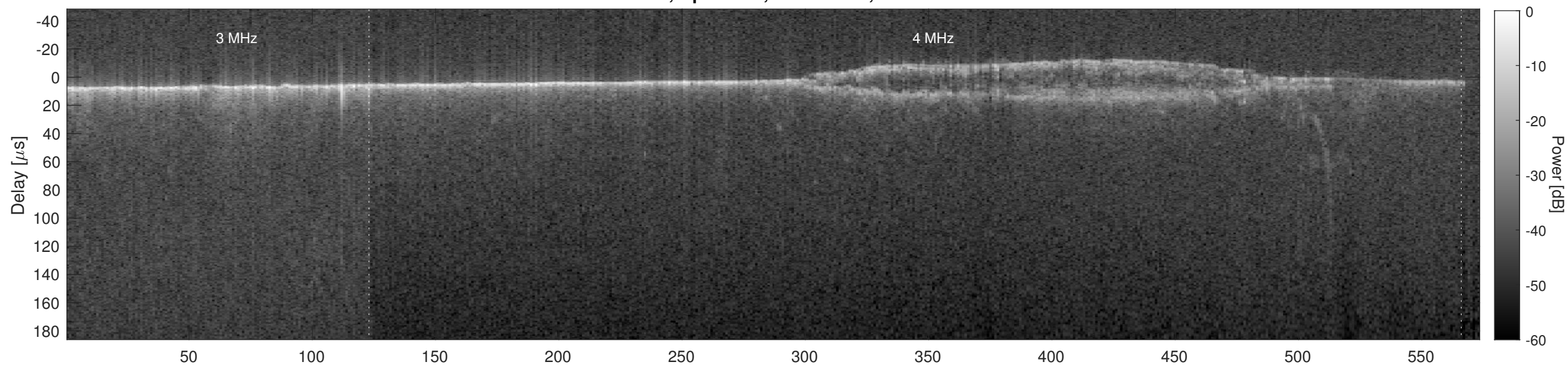
Orbit 5726, Cluttergram
