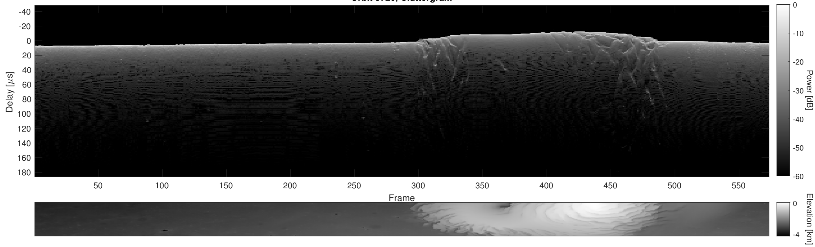
Orbit 5726, Cluttergram
