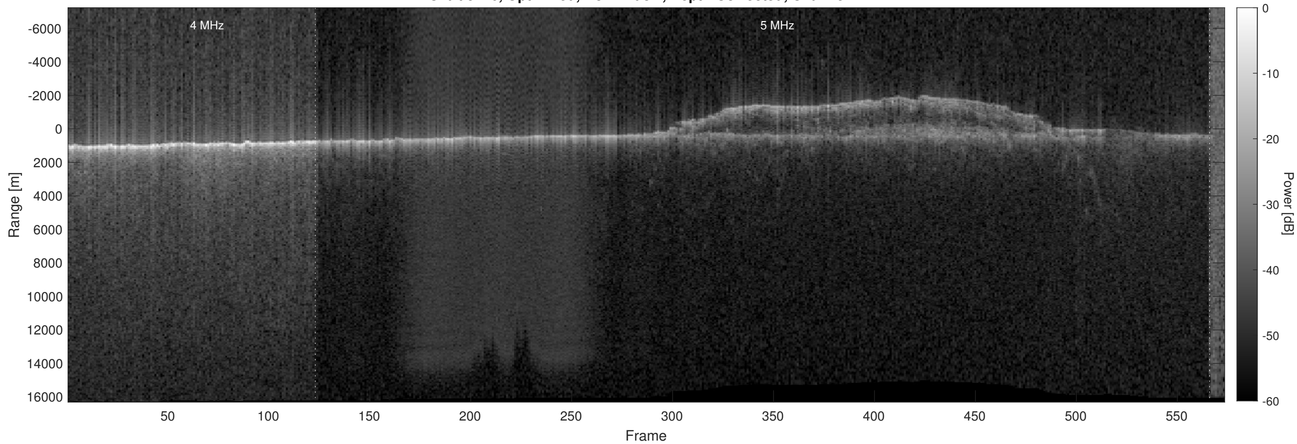
Orbit 5726, Optimized, No Window, Depth-Corrected, Channel 2
