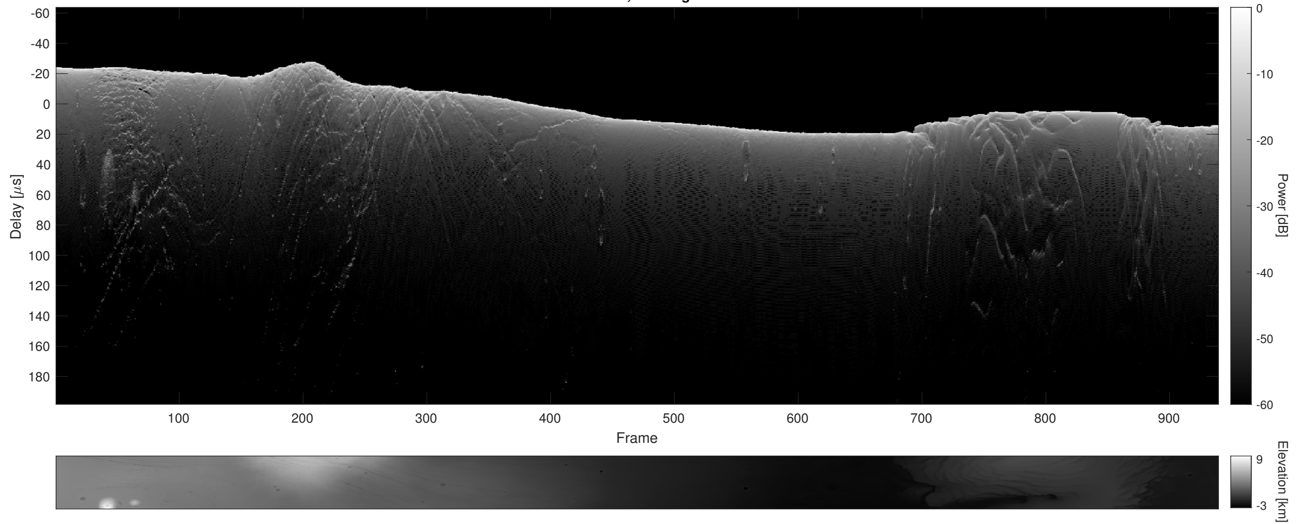
Orbit 5727, Cluttergram
