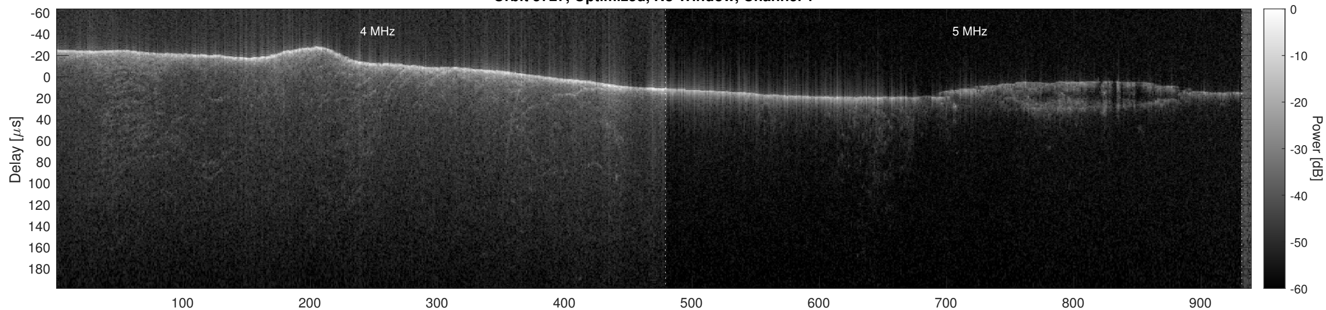
Orbit 5727, Optimized, No Window, Channel 2
