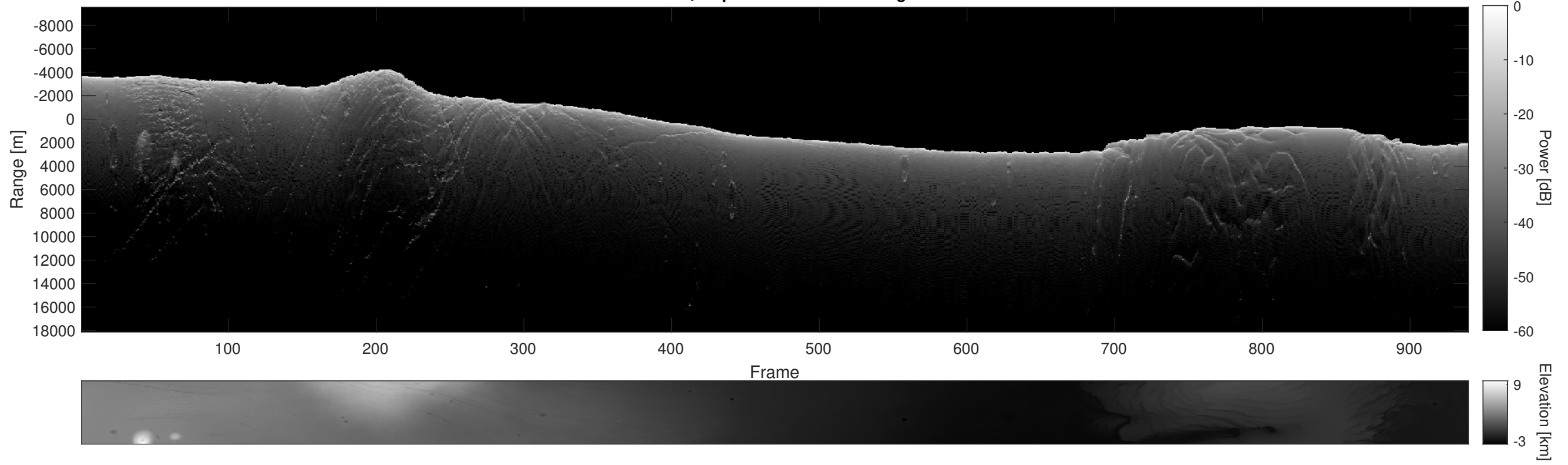
Orbit 5727, Depth-Corrected Cluttergram
