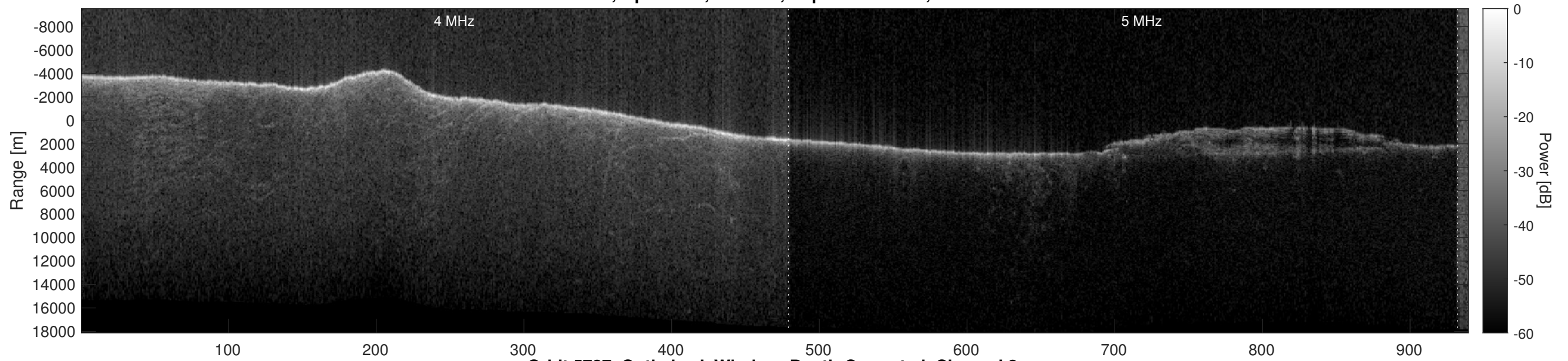
Orbit 5727, Optimized, Window, Depth-Corrected, Channel 2
