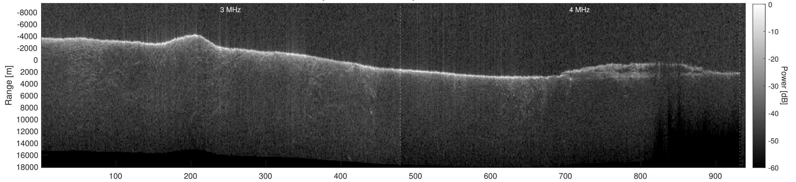
Orbit 5727, Depth-Corrected Cluttergram
