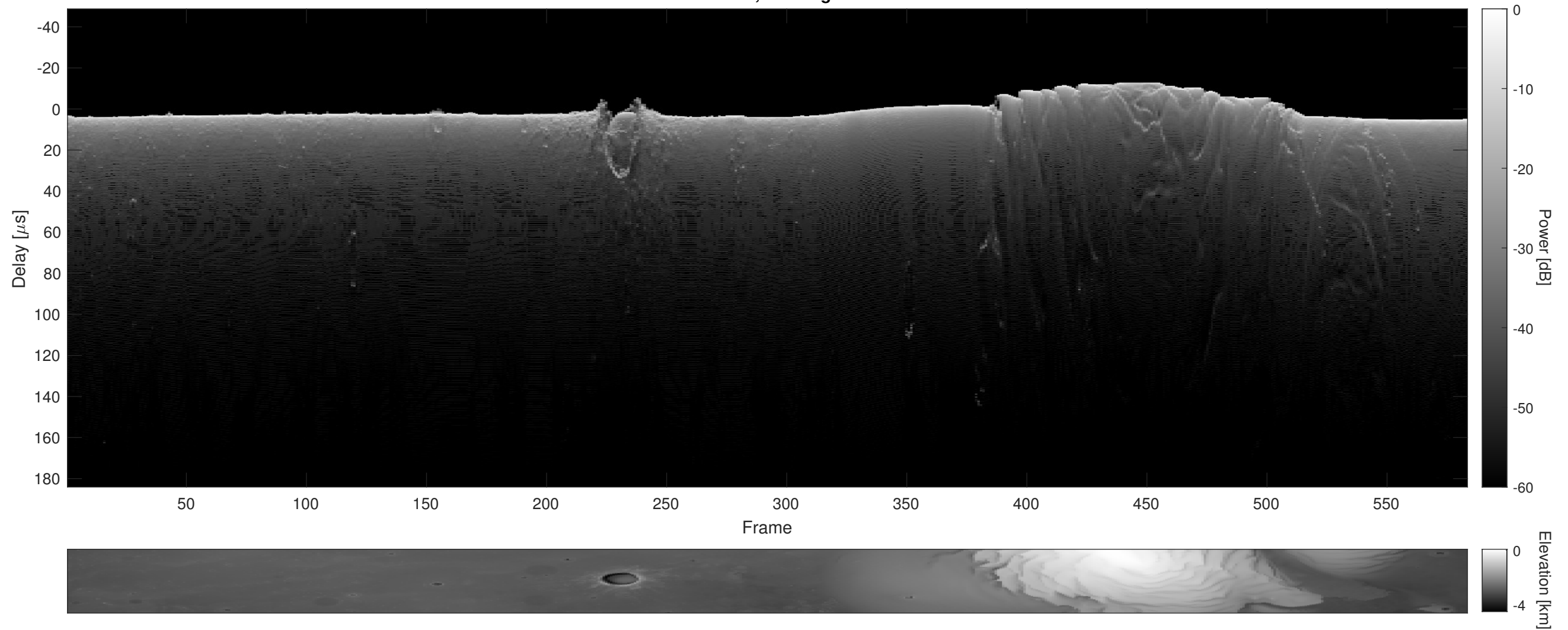
Orbit 5728, Cluttergram
