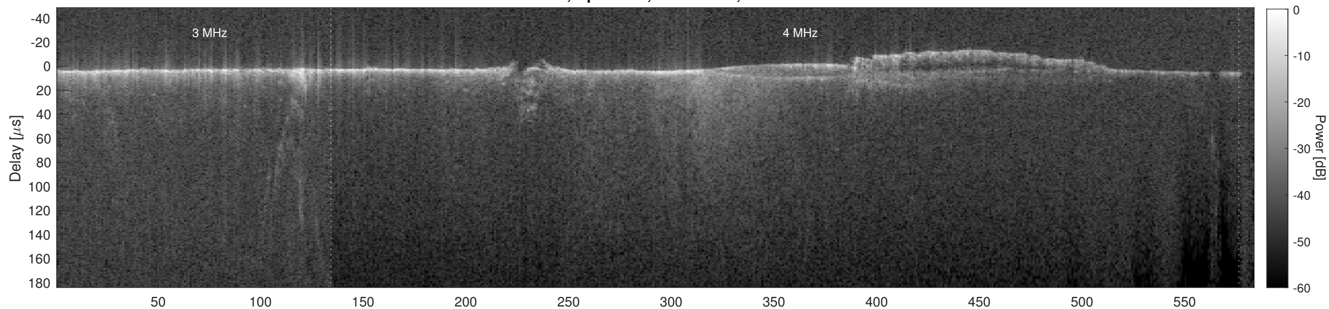
Orbit 5728, Cluttergram
