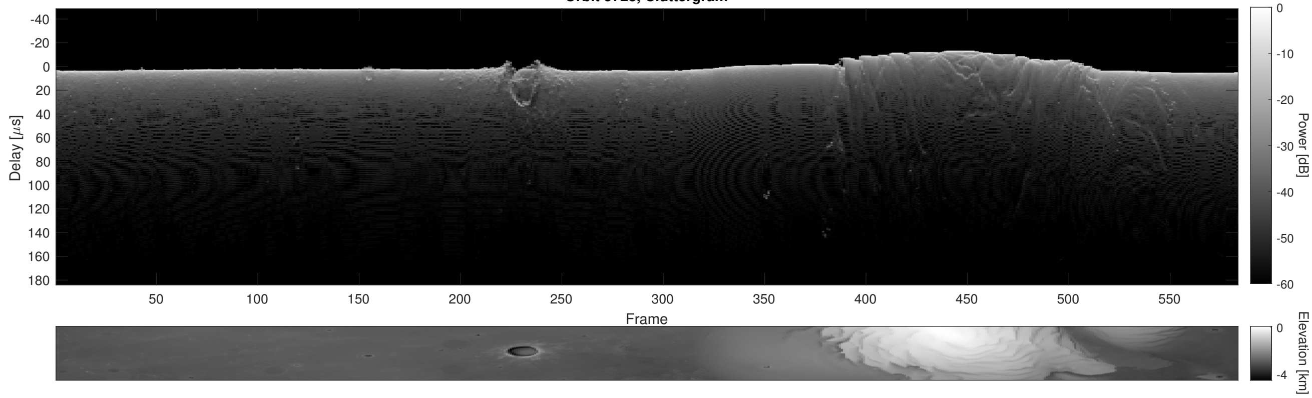
Orbit 5728, Cluttergram
