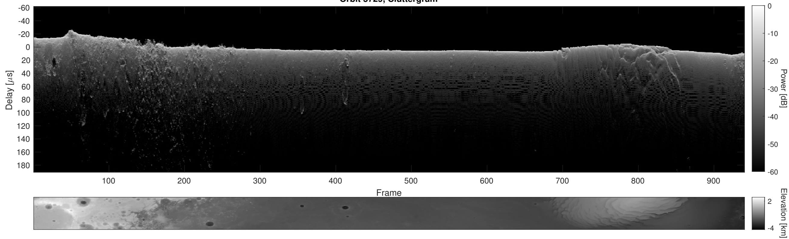
Orbit 5729, Cluttergram
