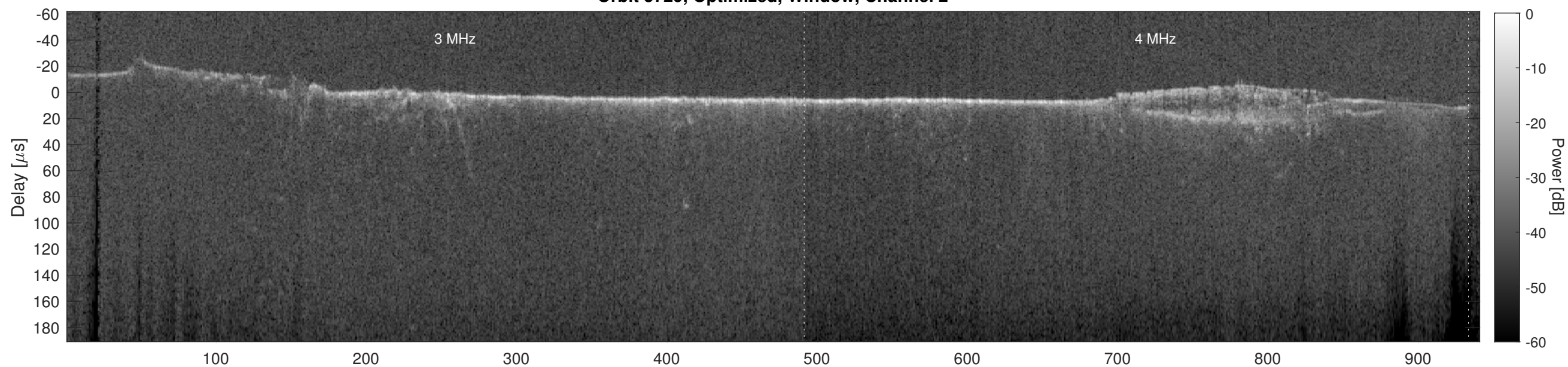
Orbit 5729, Cluttergram
