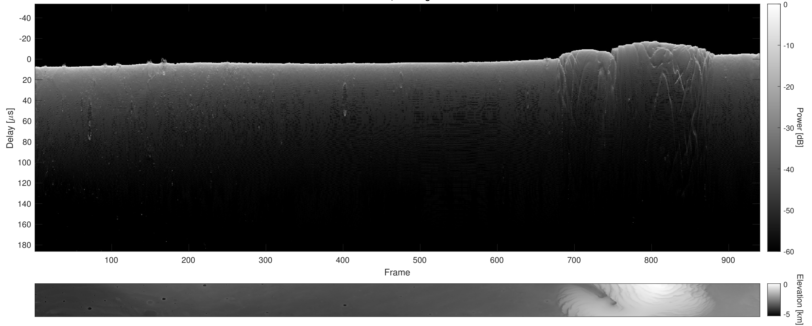
Orbit 5730, Cluttergram
