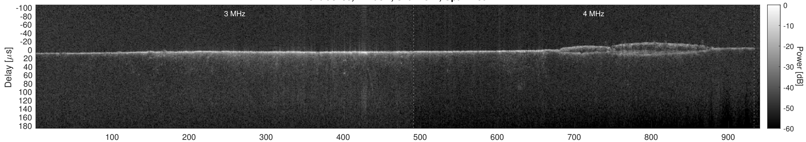
Orbit 5730, Cluttergram
