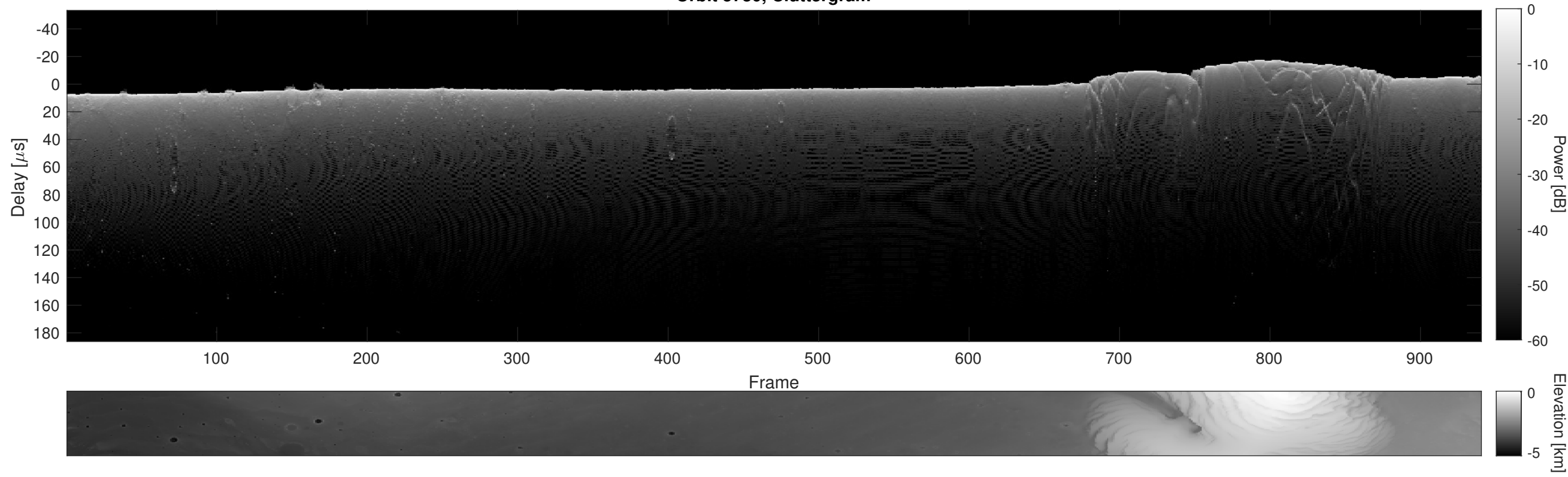
Orbit 5730, Cluttergram
