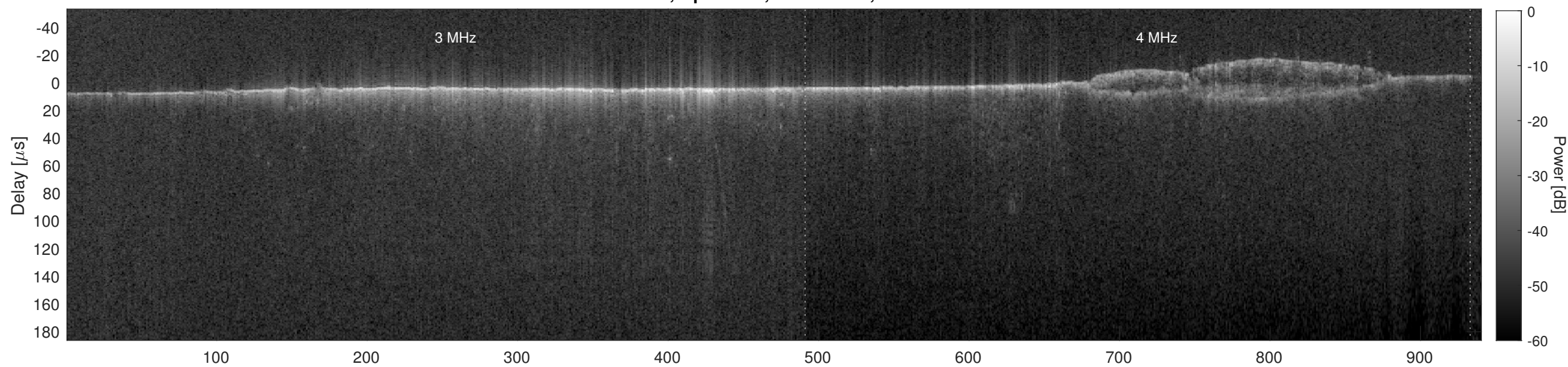
Orbit 5730, Cluttergram
