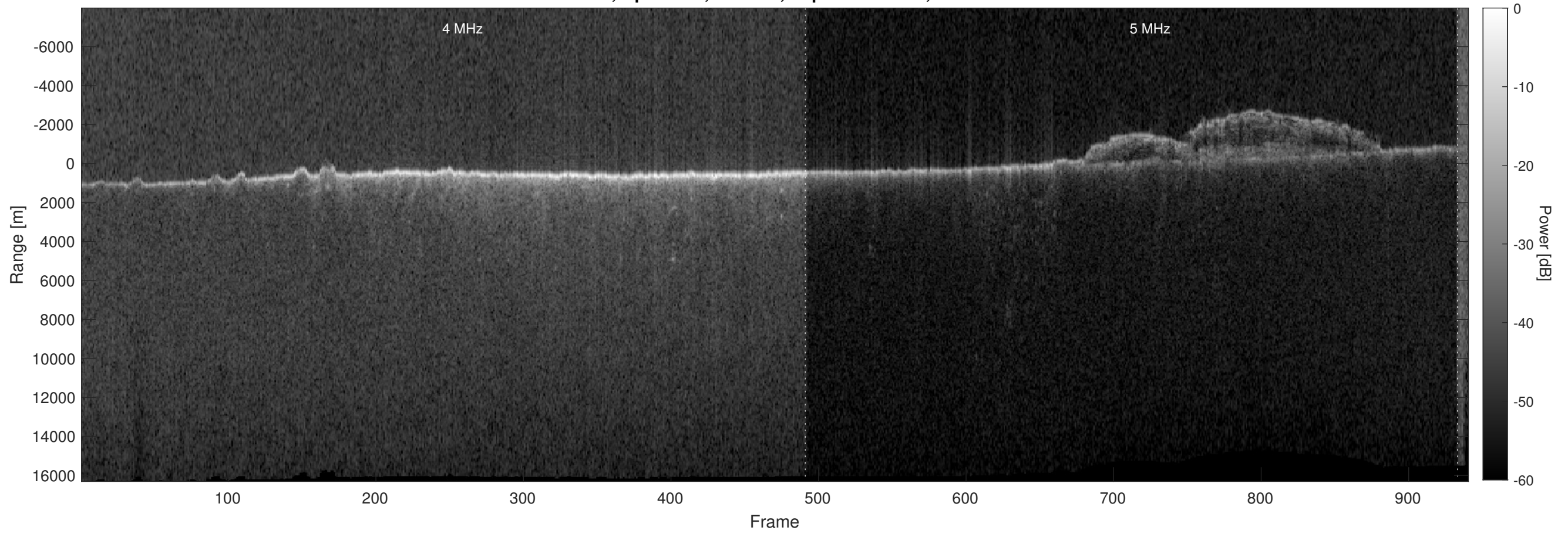
Orbit 5730, Optimized, Window, Depth-Corrected, Channel 2
