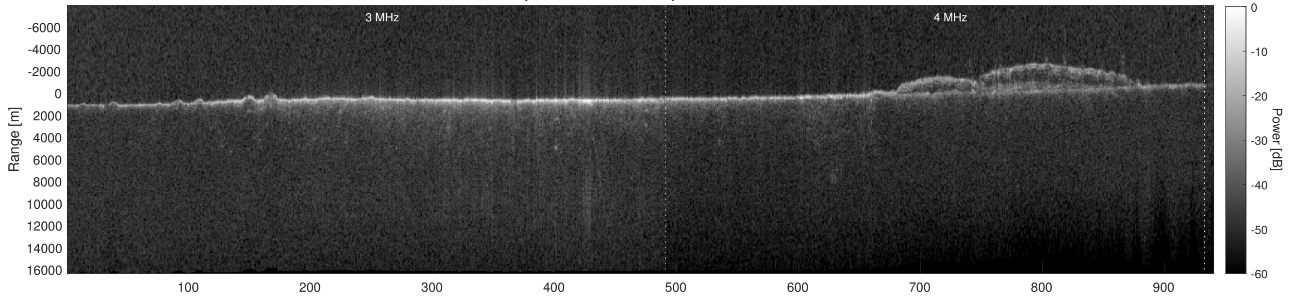
Orbit 5730, Depth-Corrected Cluttergram
